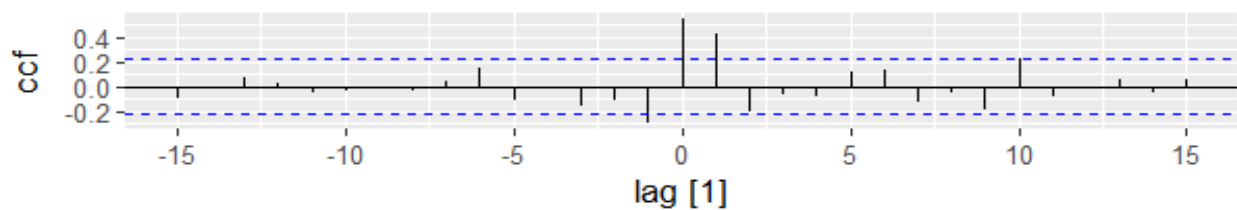
(b) 'Corona' with 'Distance learning'
