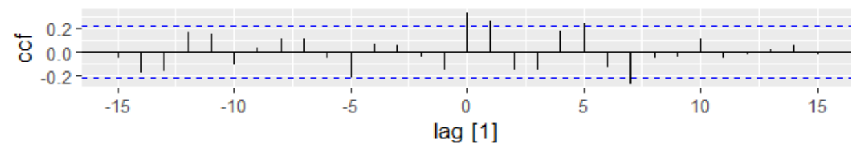
(h) 'Covid' with 'Online teaching'
