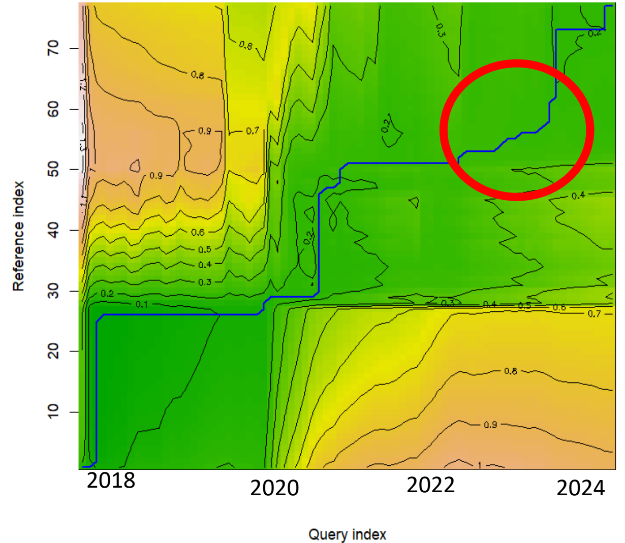
(b) Cumulative cost density with the warping path between 'Online Learning' and 'covid'
