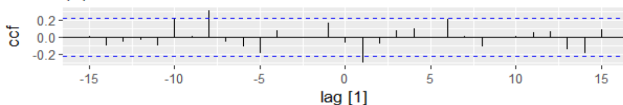
(e) 'Corona' with 'Online proctoring'
