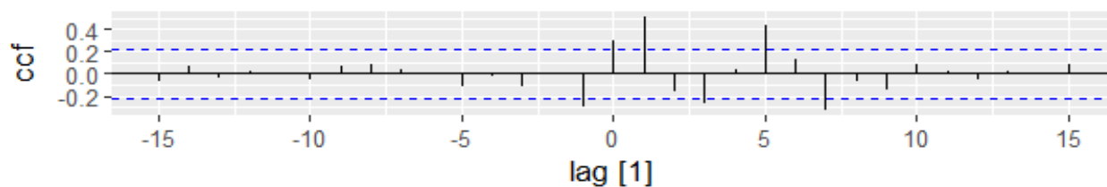
(c) 'Corona' with 'Online teaching'
