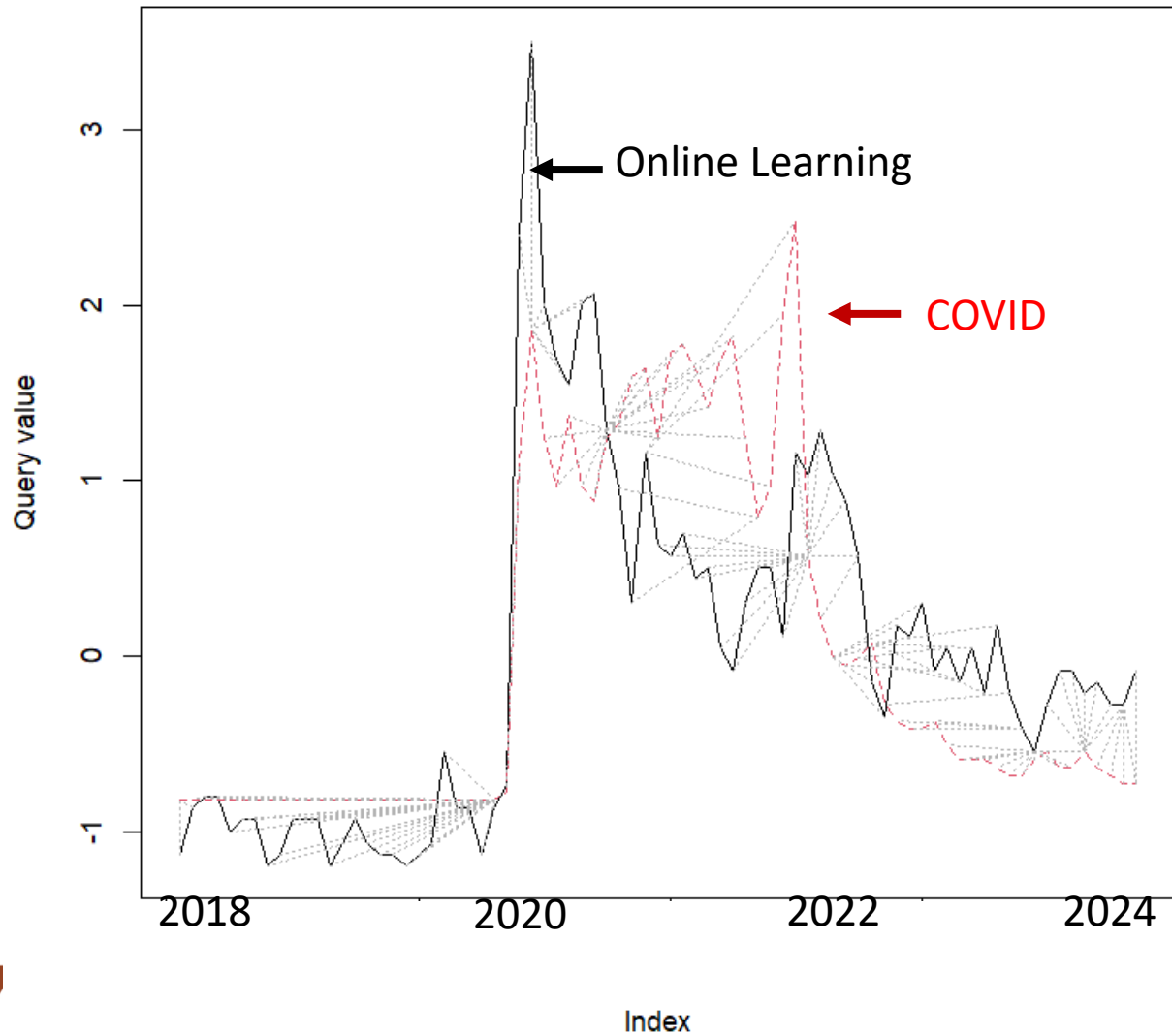
(a) Pointwise comparison between 'Online Learning' and 'covid'
